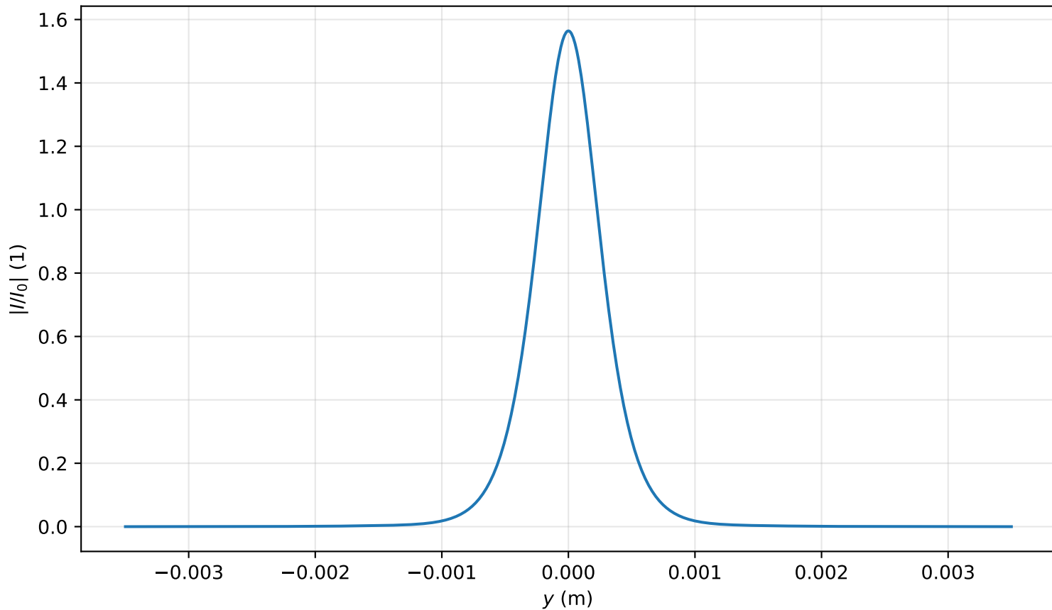
Intensity profile I(x=0, y, z=3.025)/I_0 , P_{in}=0.9P_{cr} , artificial time
